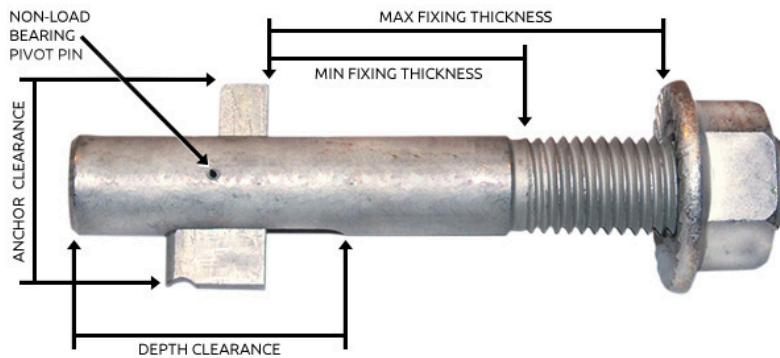
FIGURE 1—TYPICAL BLIND BOLT
